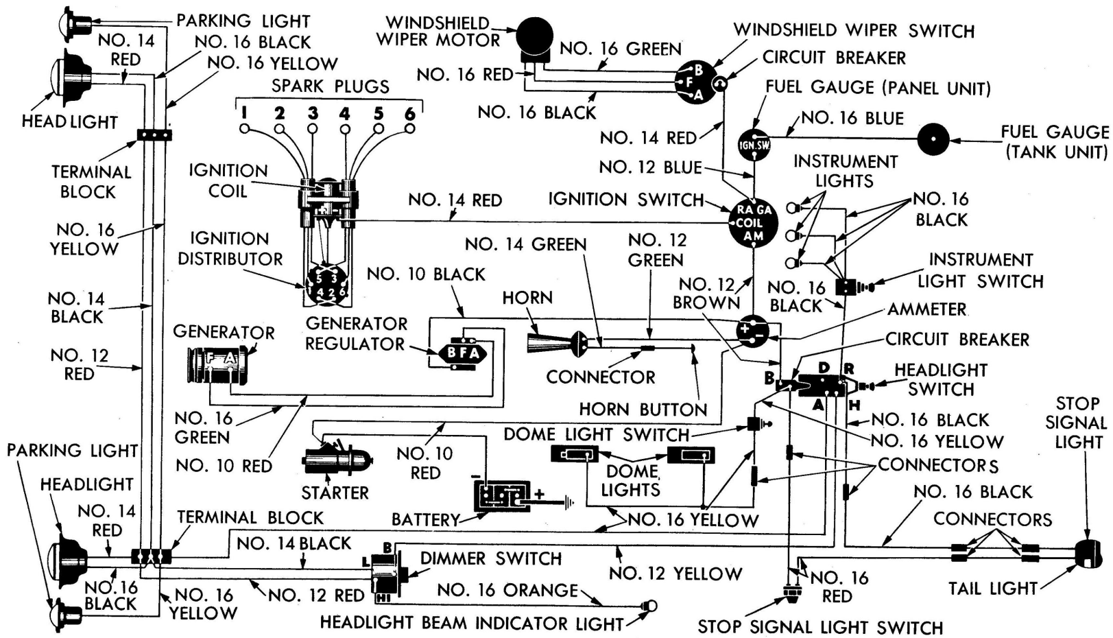
Fig. 4—Wiring Diagram (B-4-DU, B-4-EU)
