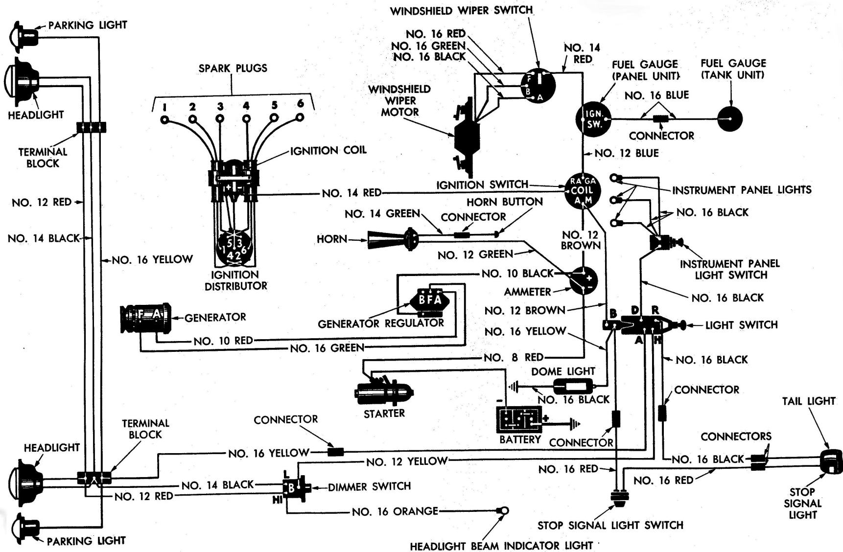
Fig. 5—Wiring Diagram (B-4-R, B-4-T, B-4-V and B-4-Y)
