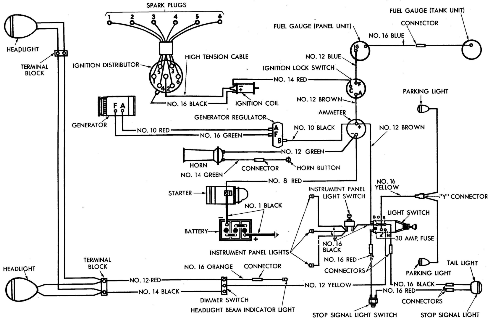
Fig. 3—Wiring Diagram (B-4-PW)
