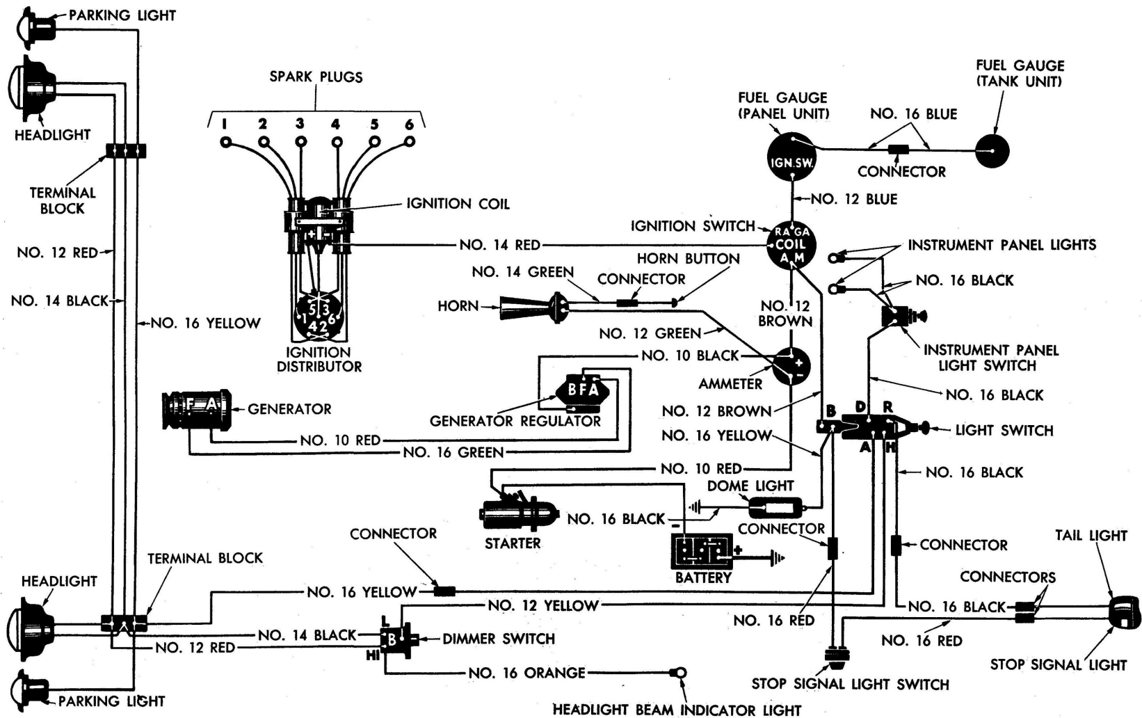
Fig. 2—Wiring Diagram (B-4-B, B-4-C, B-4-D, B-4-F, B-4-G, B-4-H, B-4-HM, B-4-J, B-4-JM, B-4-K, B-4-KMA)
